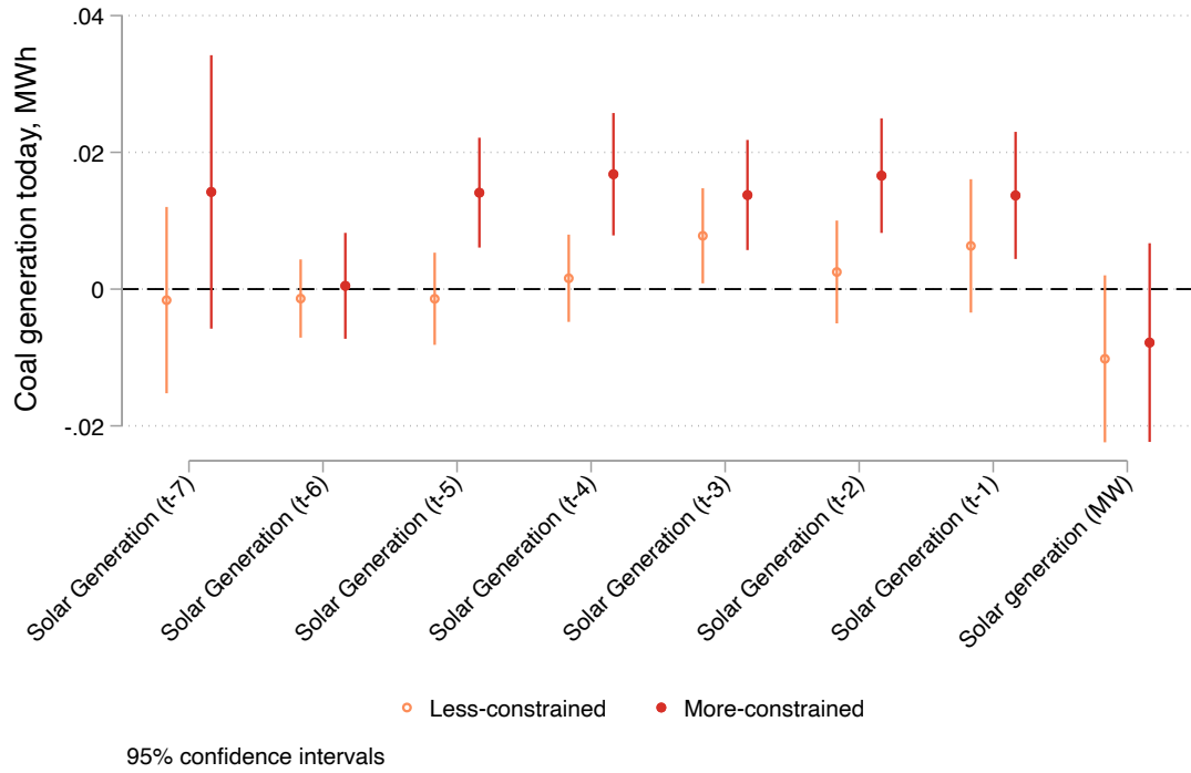
FIGURE 11. Impacts of Solar Generation on Coal-Constrained Power Plants
