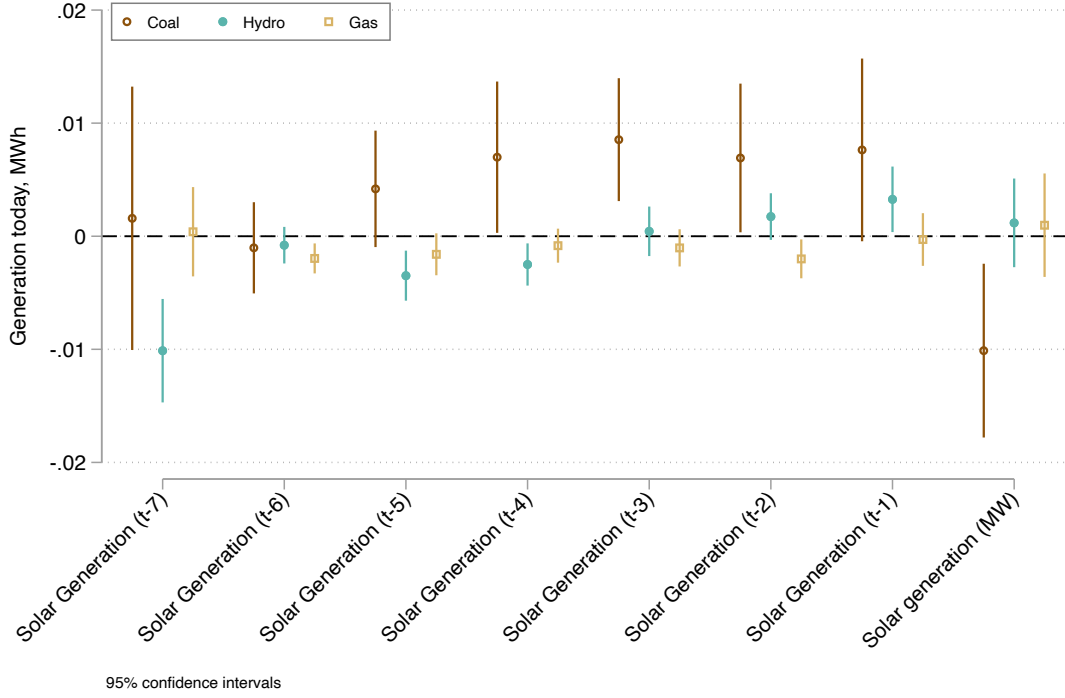
FIGURE 9. Impacts of Solar Generation on Power Plant-level Generation: By Fuel
