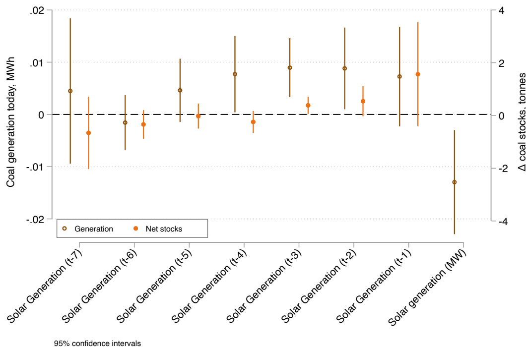
FIGURE 10. Impacts of Solar Power on Coal Stocks at Power Plants
